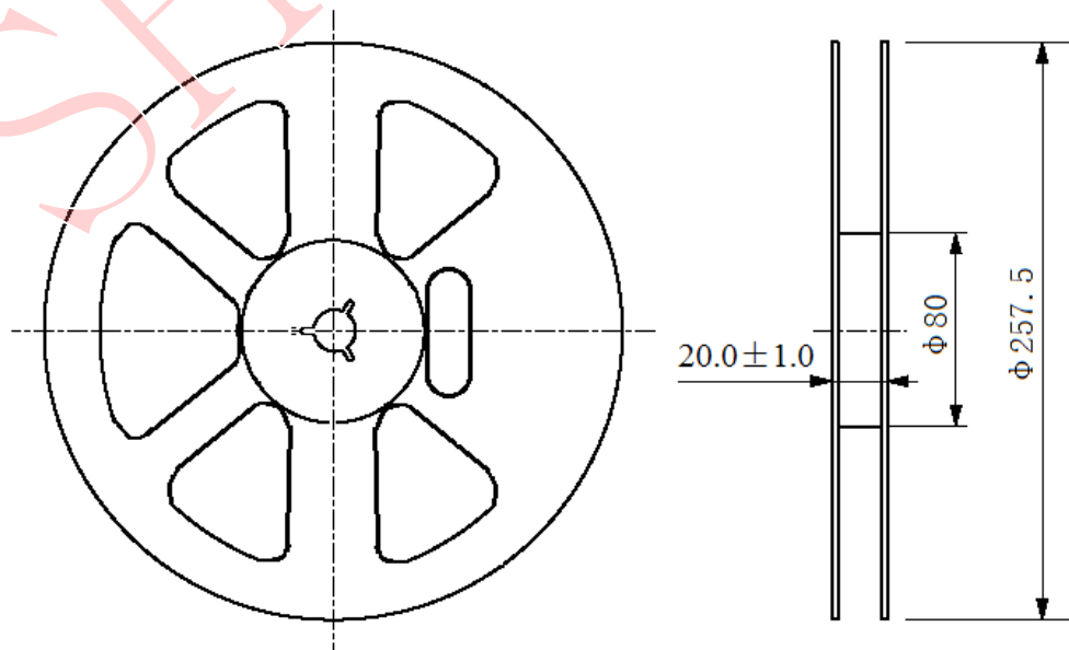
φ 257.5 Reel Dimension
